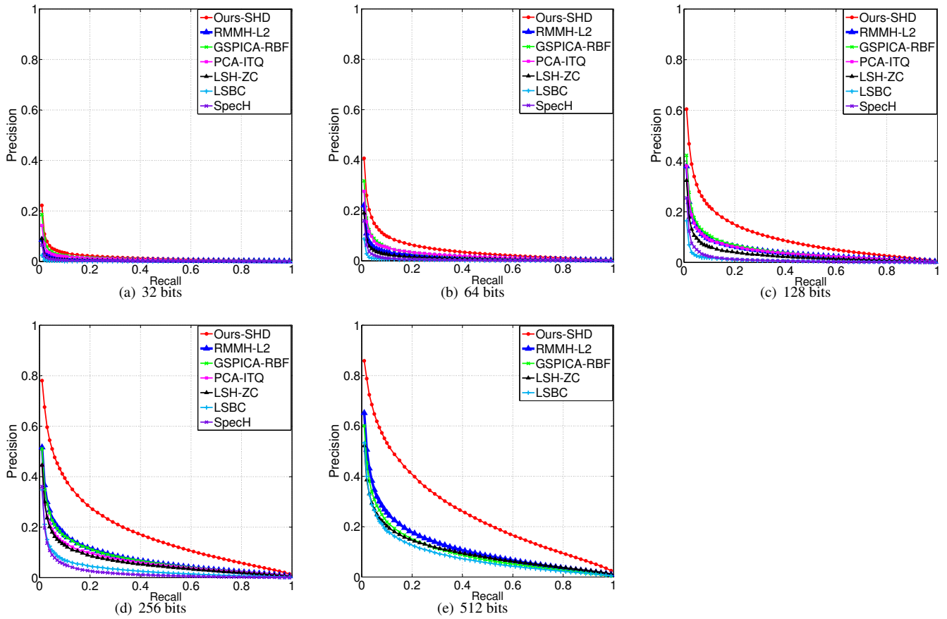
Figure 9. These graphs are precision-recall curves of tested methods with GIST-1M-384D datasets at various code length when k = 100 .
