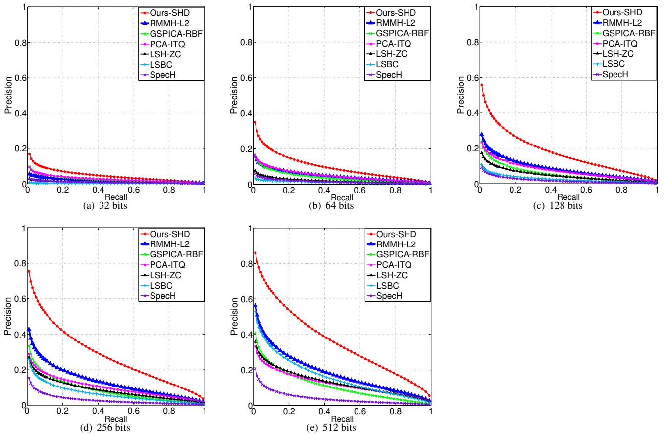
Figure 10. These graphs are precision-recall curves of tested methods with GIST-1M-960D datasets at various code length when k = 1000 .
