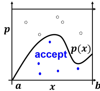
Figure 9.3: In the rejection method, we generate random numbers and accept numbers only when those numbers are within the pdf p(x) .
