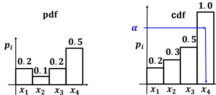
Figure 9.2: This figure shows a pdf and its cdf. Using the inverse cumulative distribution function generates samples according to the pdf by utilizing its cdf.
