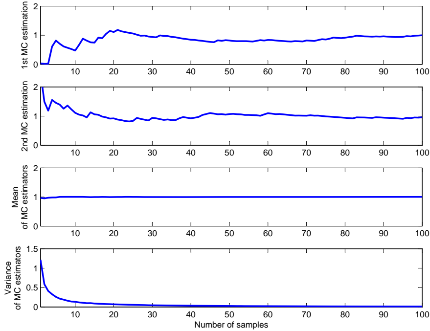
Figure 9.1: The top two sub-figures show the first and second MC estimators of \int_0^1 4x^3 dx , whose ground truth value is 1. These MC estimators approach to their ground-truth, as we have more number of samples. While these individual MC estimators have up and down depending on their randomly generated values, their mean and variance measured with 600 estimators show the expected behavior, as theoretically predicted in Sec. 9.1. Its source code, mc_int_ex.m , is available.
